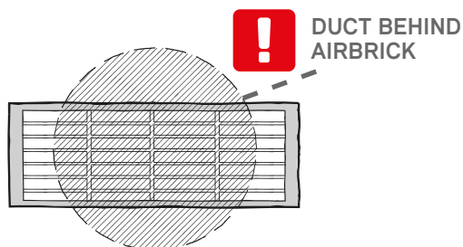
CLAY AIR BRICK DOES NOT HAVE ENOUGH FREE AREA
