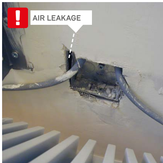
RADIATOR SEAL PROBLEMS - POOR SEAL
